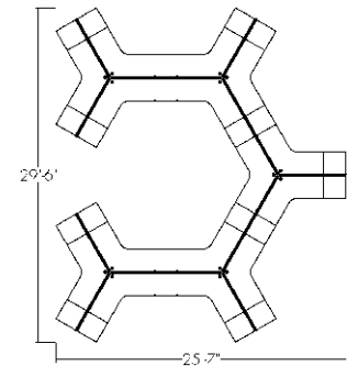
End / Mid / inner cube 9x9 / 9x6½ / 6½x6½
