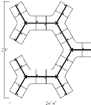
End / Mid / inner cube 9x9 / 9x6 / 6x6
