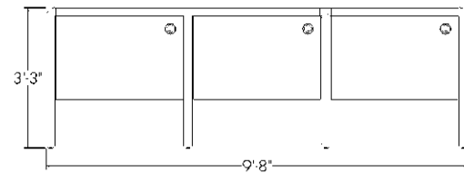
4x3 Ref: CC-08-4x3
