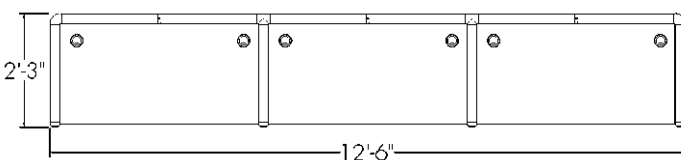
4x2 Ref: CC-08-4x2
