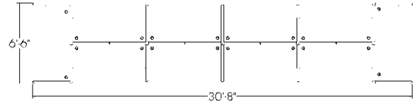
6x3 Ref: CC-13-6x3
